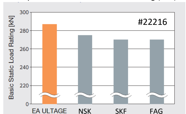
Comparison of basic static load rating (Cor)
