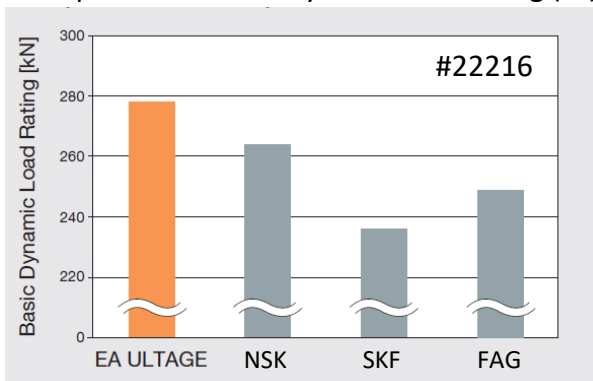
Comparison of basic dynamic load rating (Cr)
