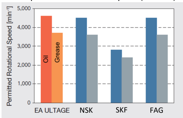
Comparison of allowable speed (#22216)
