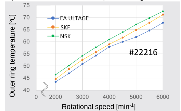
Temperature rise test result (circulating lubrication)
